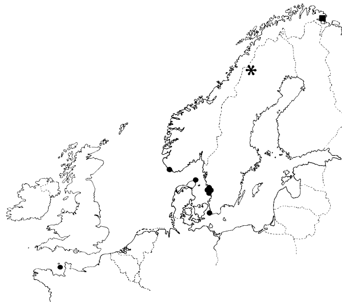
Figure 1. Recoveries of Shorelarks ringed as nestlings or breeding adults at Ammarnäs in southern Lapland. Star = the ringing site. Dots = recoveries in the non-breeding season (October–April). Square = late summer recovery.
